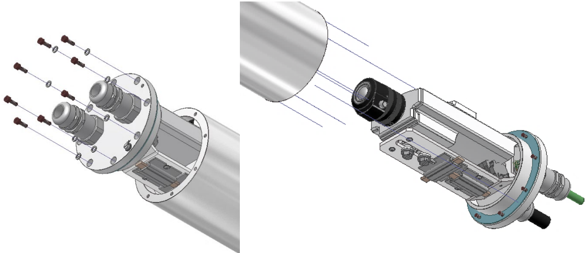
Figure 6-3 Opening the ExCam IPM1137-LE (similar illustration)
