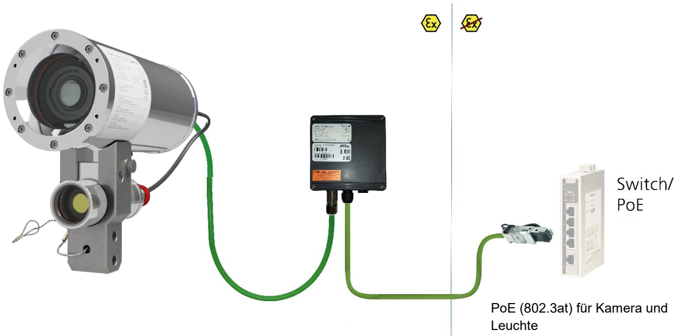
Figure 5-7 ExTB-3 -> Safe area
