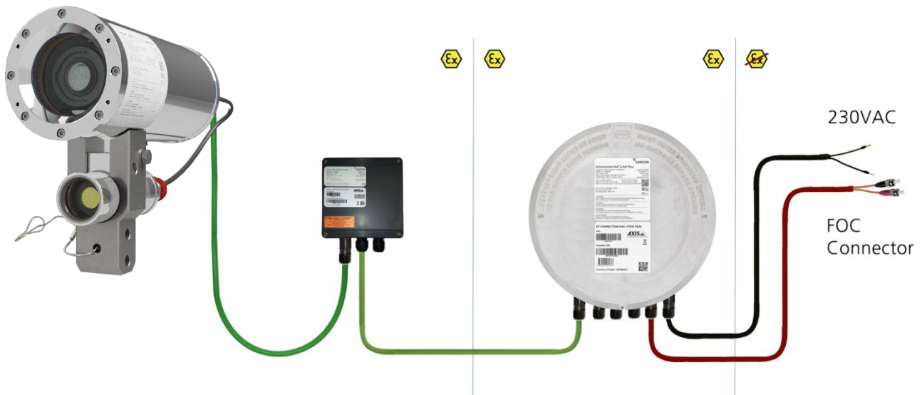
Figure 5-8 ExTB-3 -> ExConnection Rail
