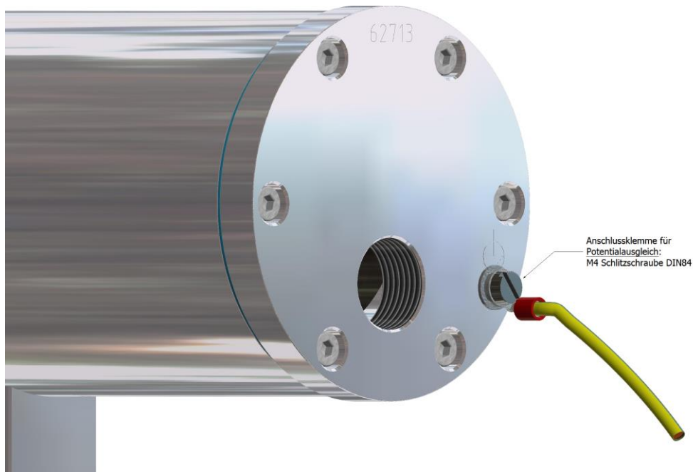
Fig. 6-7: Example terminal for potential equalization
