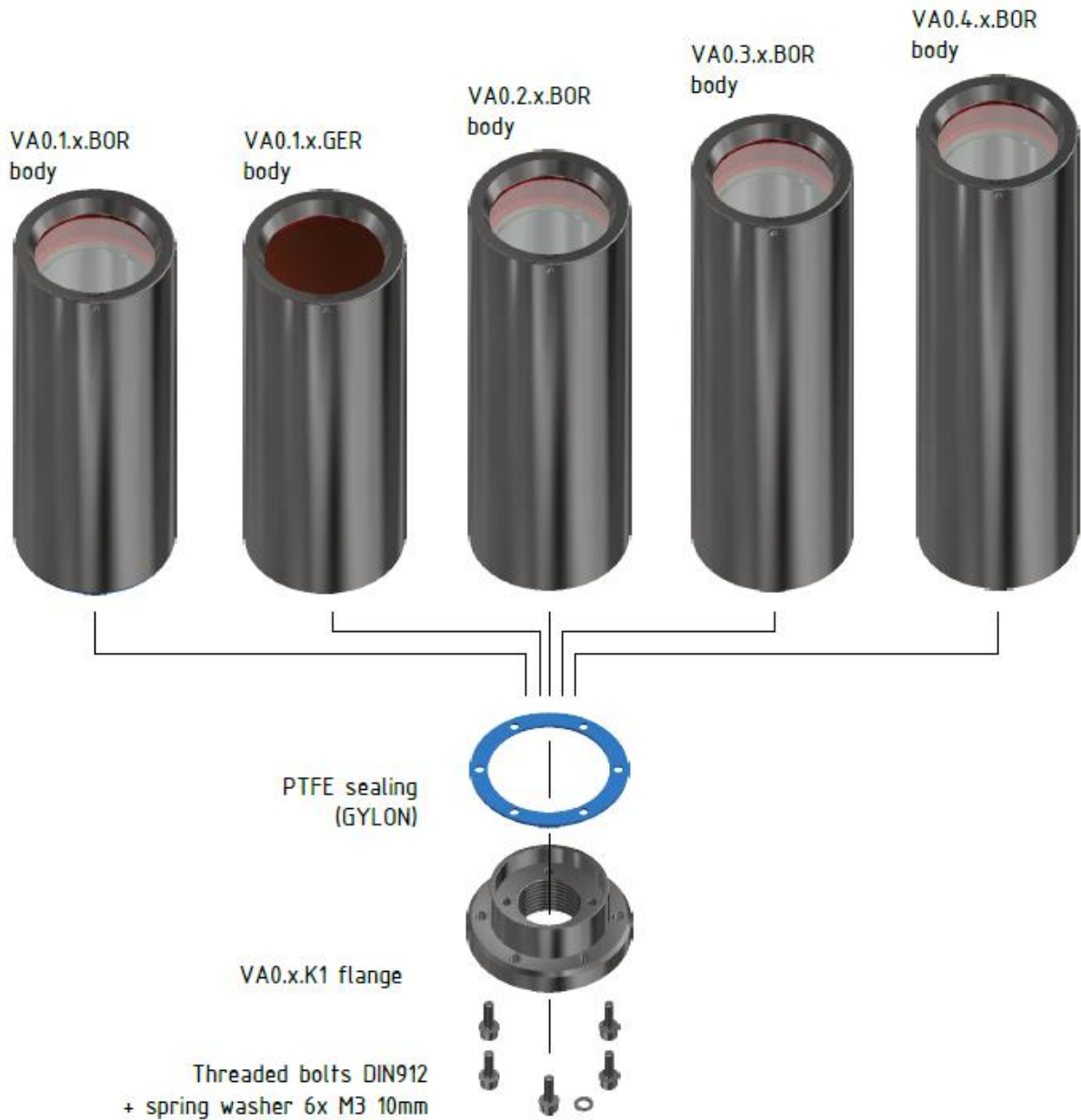
Fig. 6-1: Configuration example of the T07-VA0.x enclosure-combination
